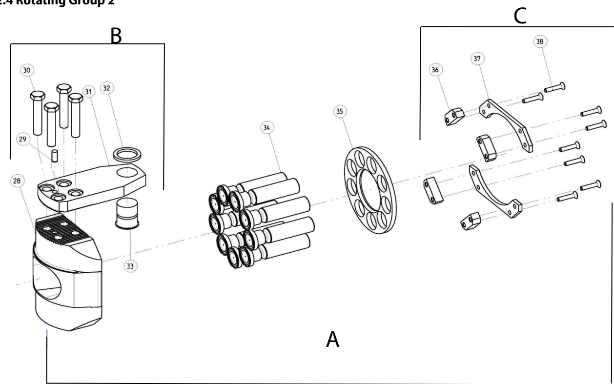
Pump size 130 ... 360
