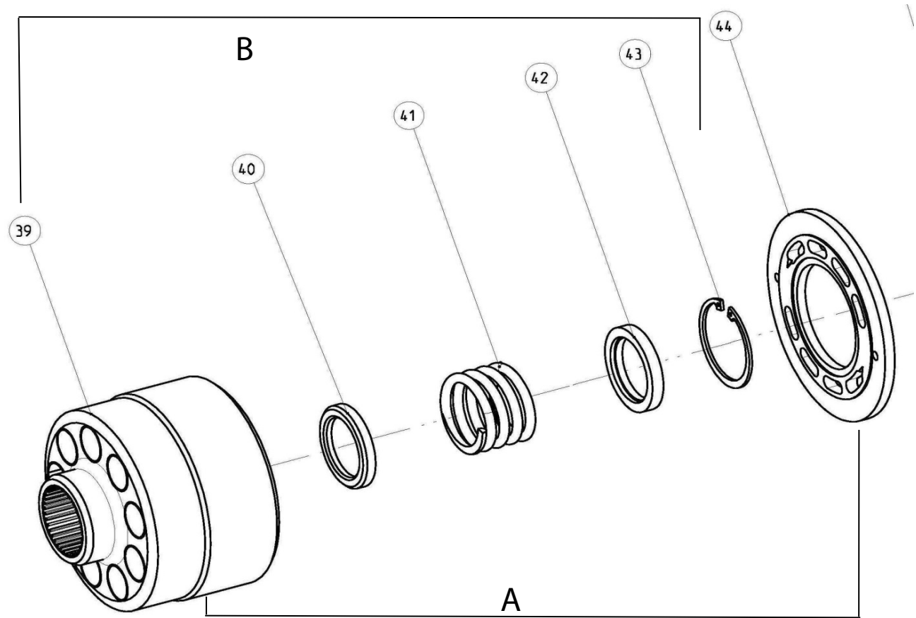
Pump size 130 ... 360
