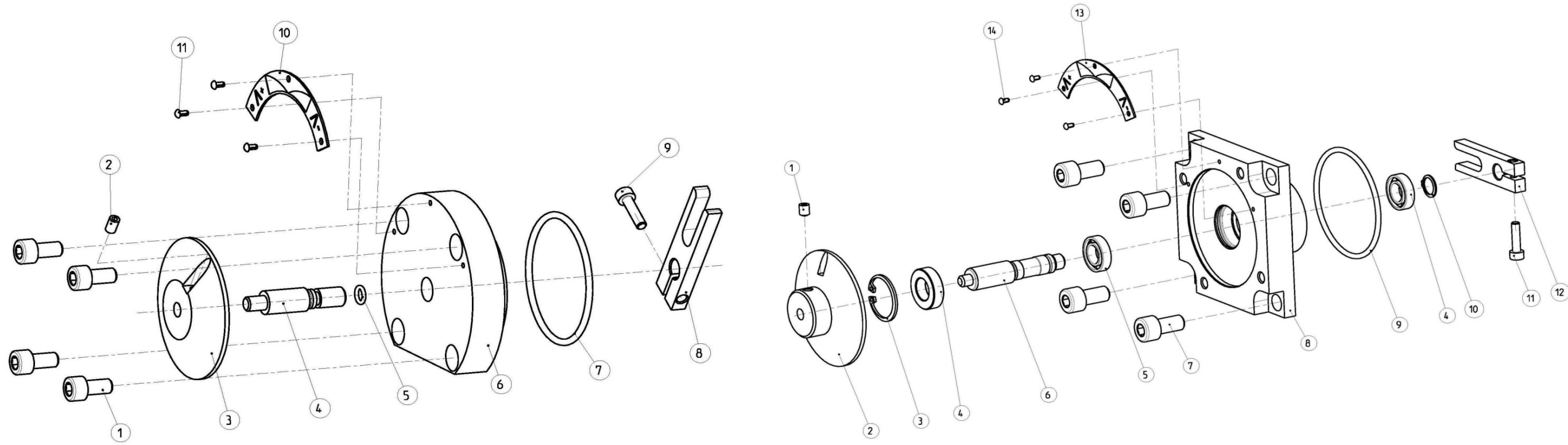
Pump size 130 ... 360
