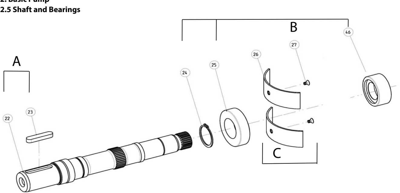
Pump size 130 ... 360
