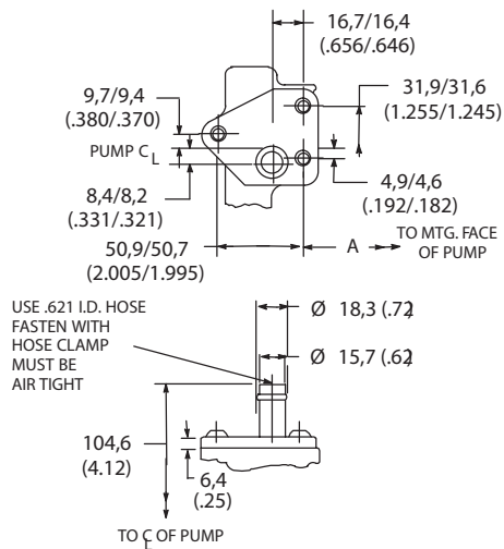
"MF" MANIFOLD
