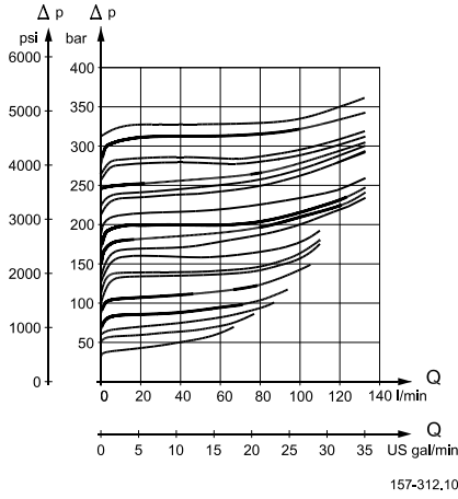
PVLP, shock valve characteristic
