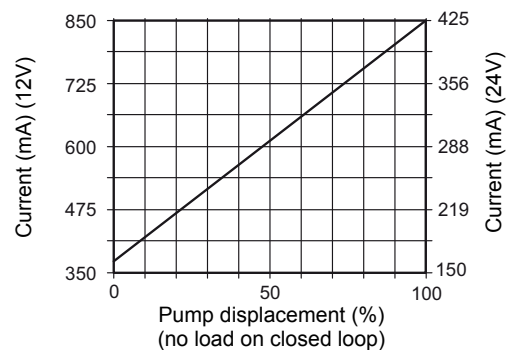
Electrovalve current vs Displacement
