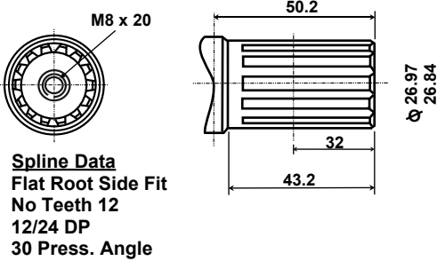
Splined Shaft - SS
