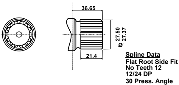
Splined Shaft - SS
