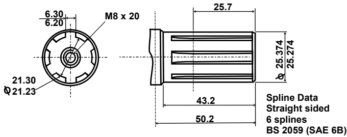
Splined Shaft - SP
